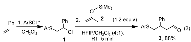
Scheme 1. \beta -Arylthioalkylation of Si-capped \pi donors. TMS = trimethylsilyl; HFIP = 1,1,1,3,3,3-hexafluoro-2-propanol.
